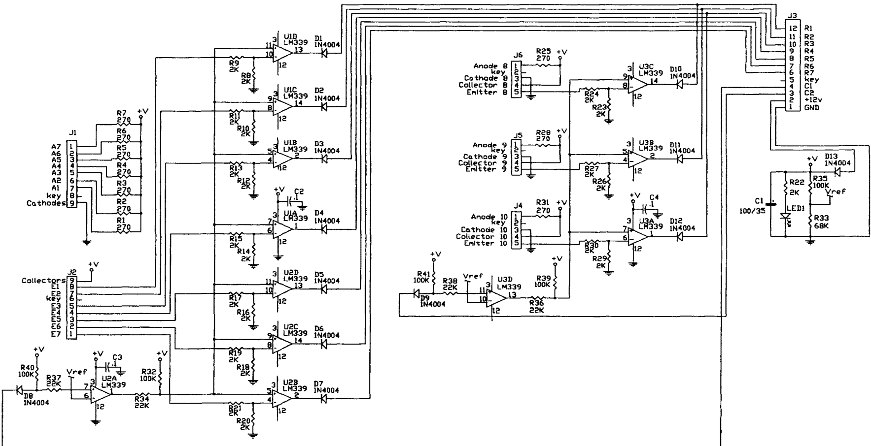
10-Opto Switch Board Schematic A-18159.1
