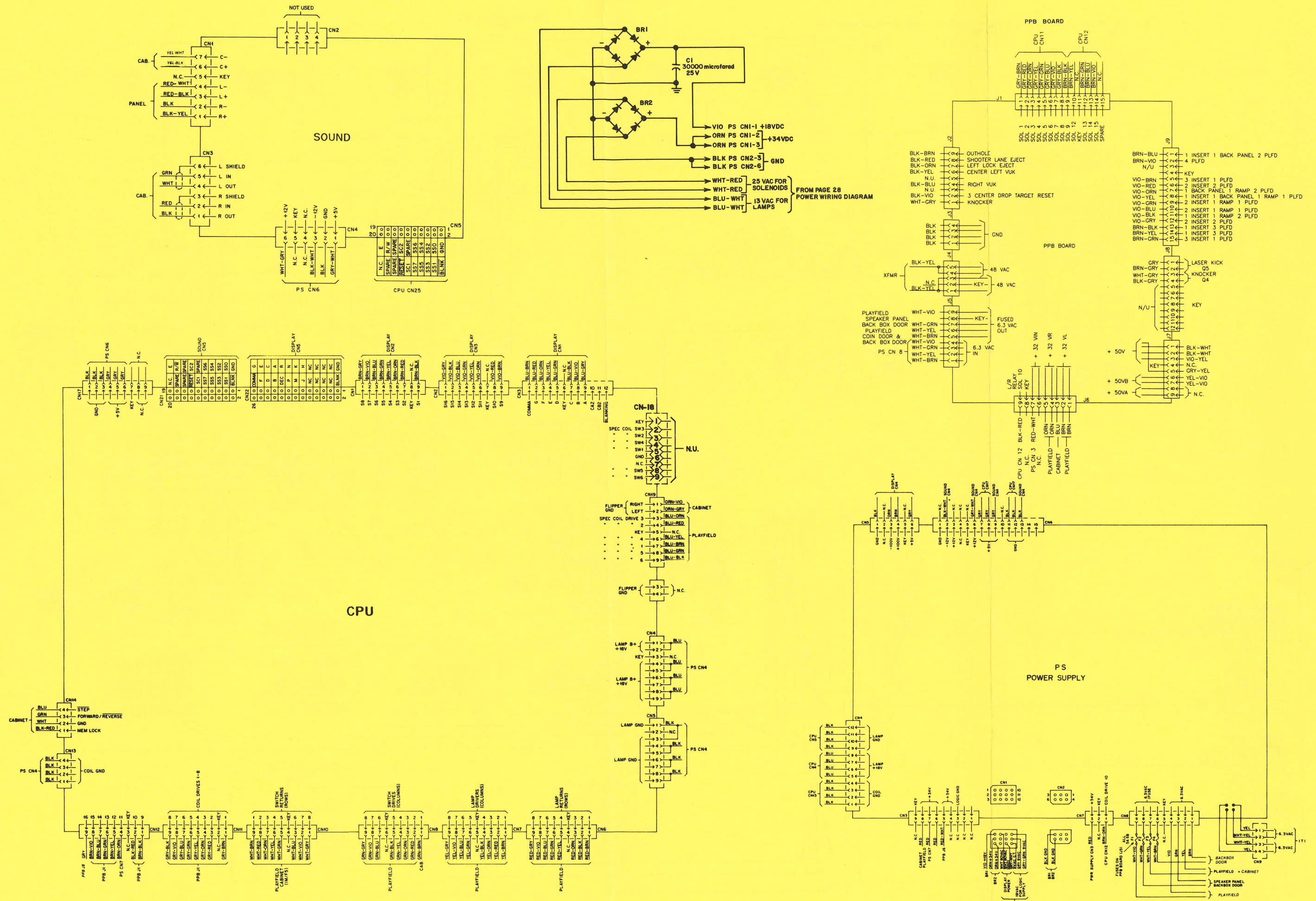
Backbox Wiring Diagram 41
