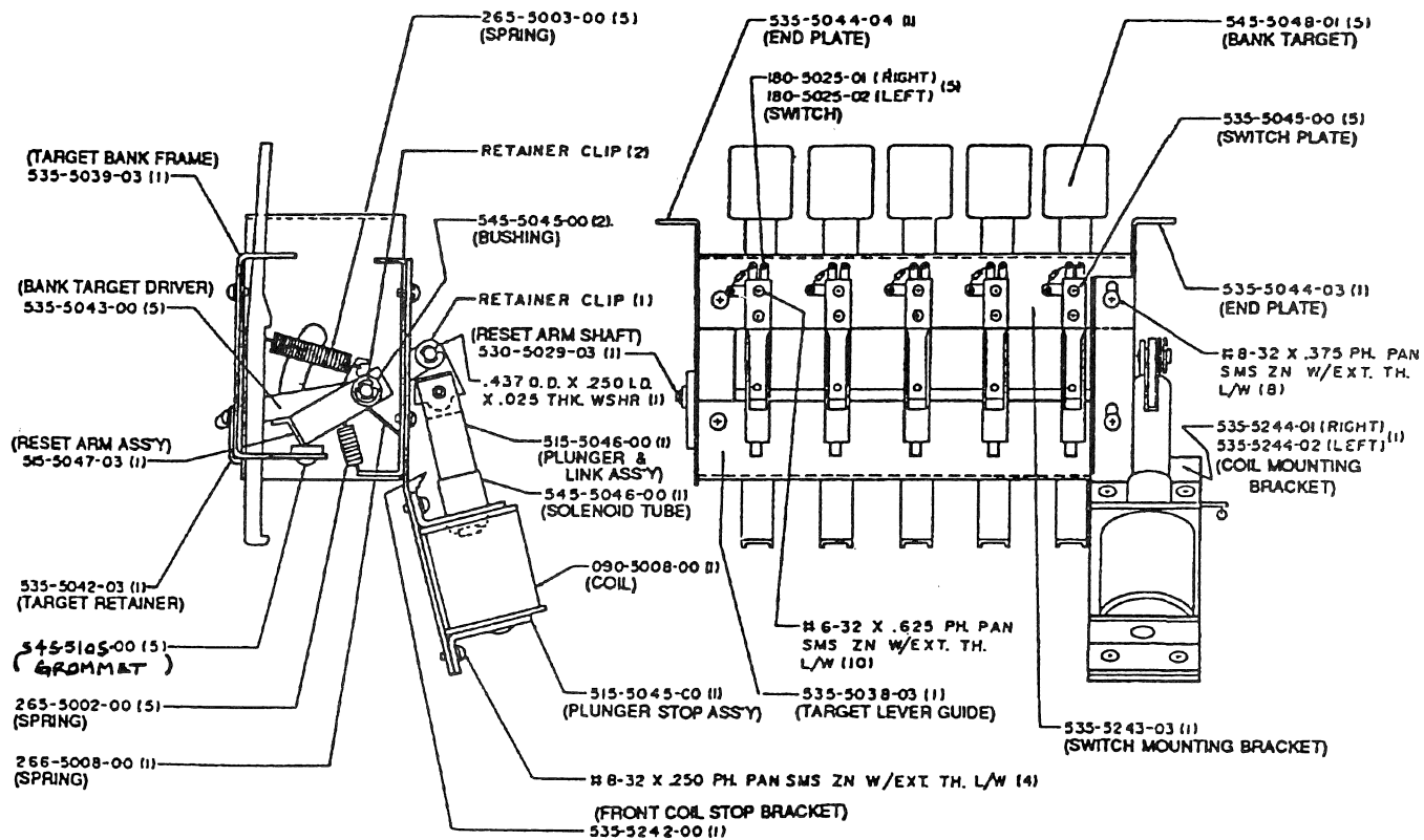
300-3055-51 (RIGHT) 5 BANK DROP TARGET -52 (LEFT) 5 BANK DROP TARGET
