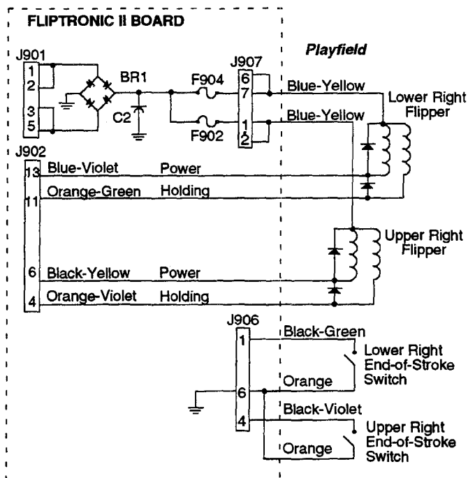
Right Flipper Circuit
