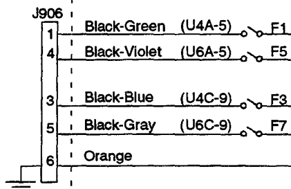
FLIPTRONIC II BOARD
