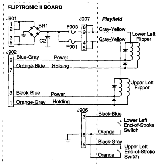
Left Flipper Circuit
